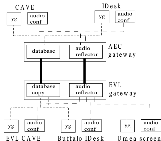
Figure 8: Network connections for Ars Electronica show
